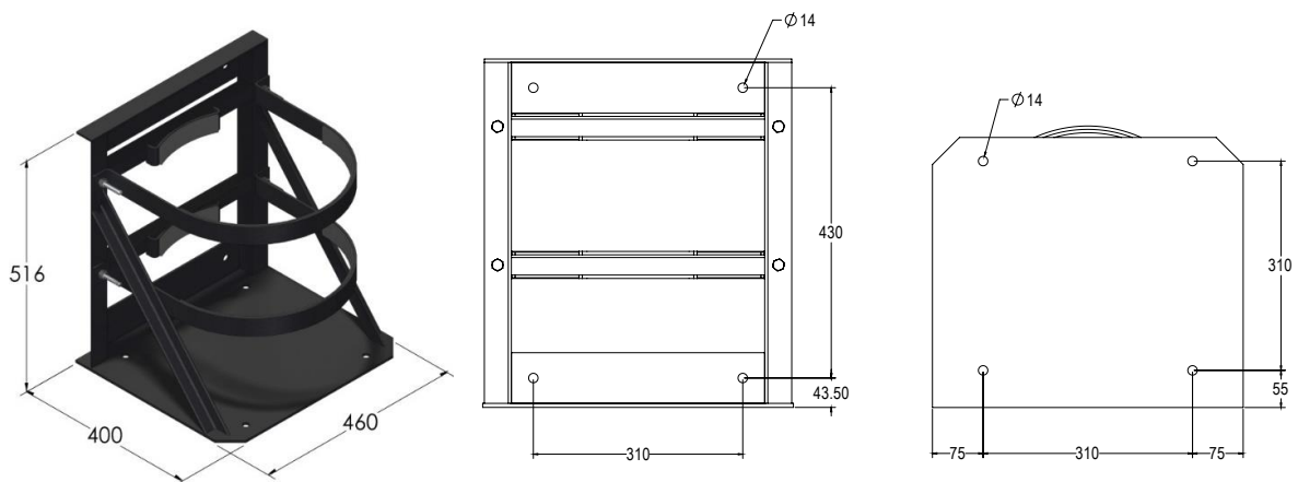
128737 – C45 & C65 Cylinder Bracket
