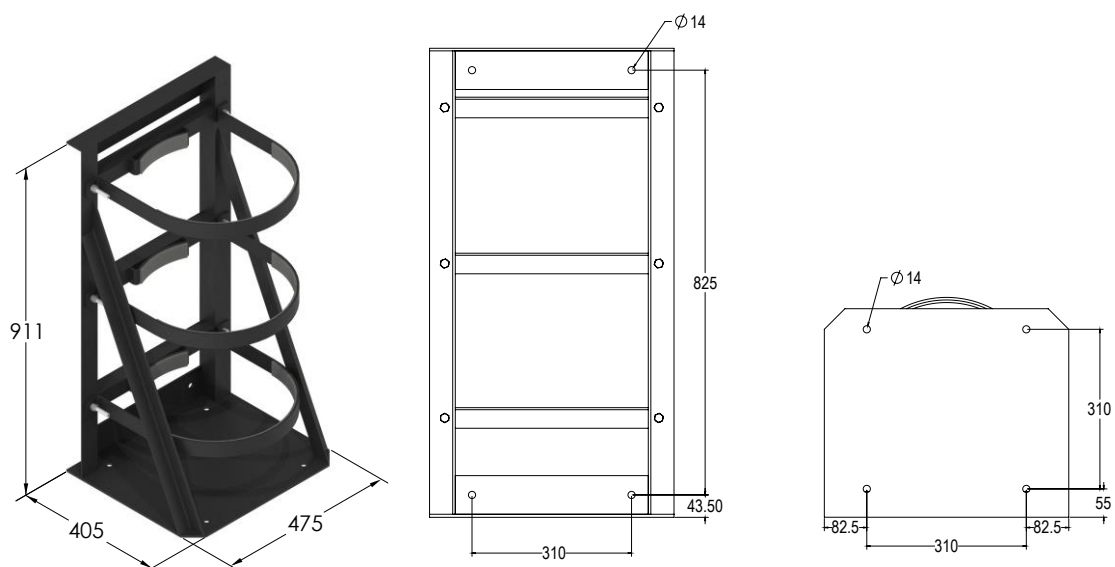
128738 – C106 Cylinder Bracket
