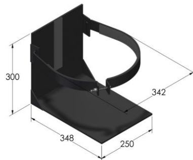
128736 – C30 Cylinder Bracket
